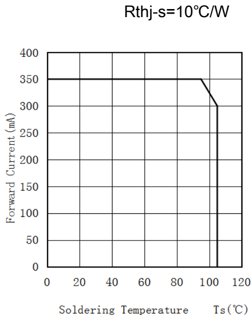
Soldering Temperature VS Allowable Forward Current 焊盘温度与允许温度电流特性
