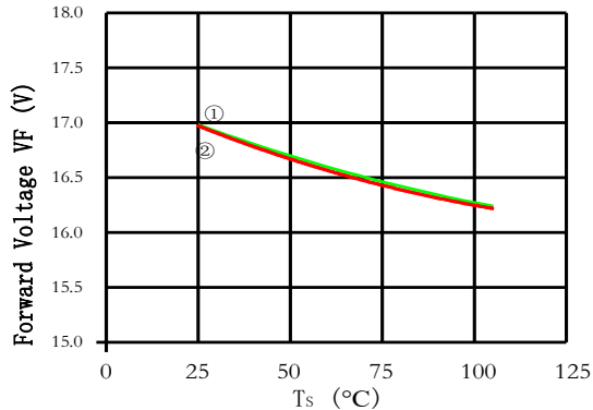
Case Temperature vs. Forward Voltage 结点温度与正向电压曲线图 IF=400mA
