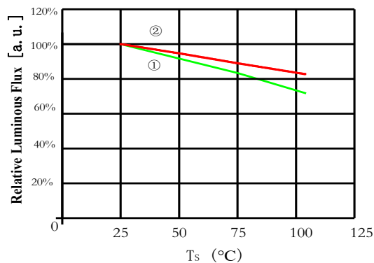
Case Temperature vs. Relative Luminous Flux 结点温度与相对流明曲线图 IF=400mA
