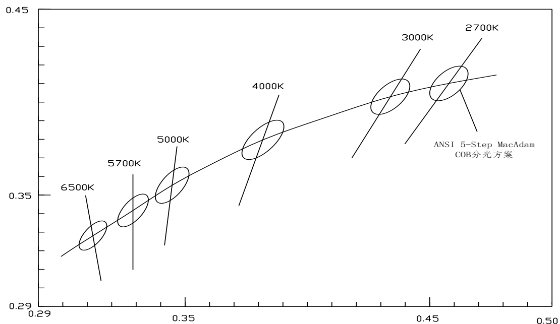
Chromaticity bins
