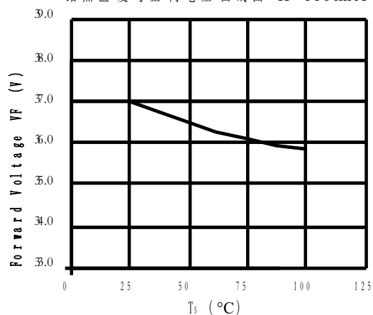
Case Temperature vs. Forward Voltage 结点温度与正向电压曲线图 I_f=1100\text{mA}
