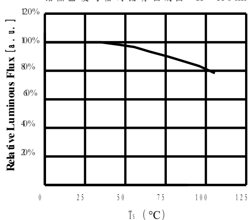
Case Temperature vs. Relative Luminous Flux 结点温度与相对流明曲线图 I_f=1100\text{mA}
