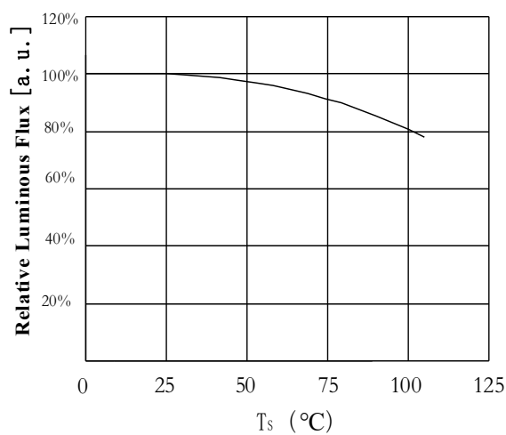
Case Temperature vs. Relative Luminous Flux 结点温度与相对流明曲线图 I_F = 850\text{mA}
