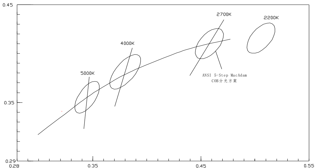
Chromaticity bins
