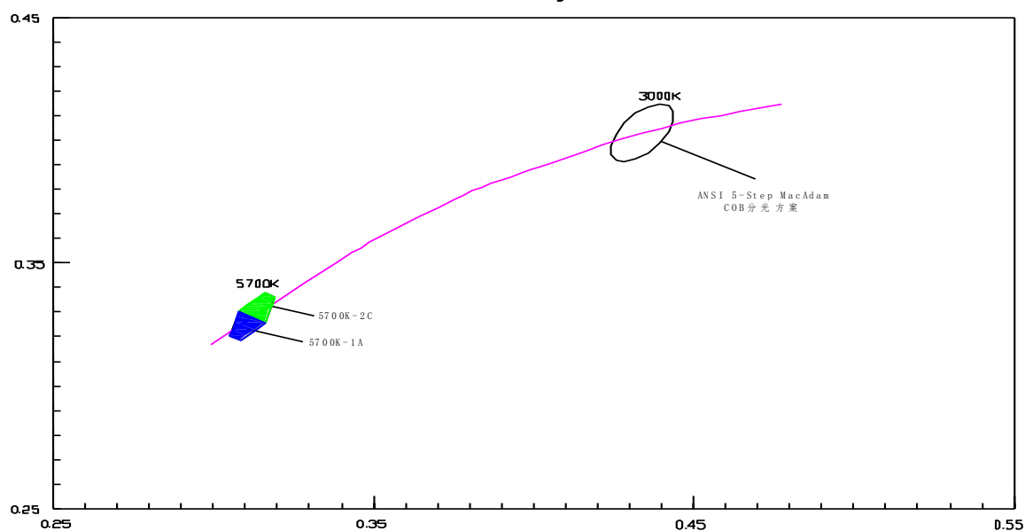
Chromaticity bins
