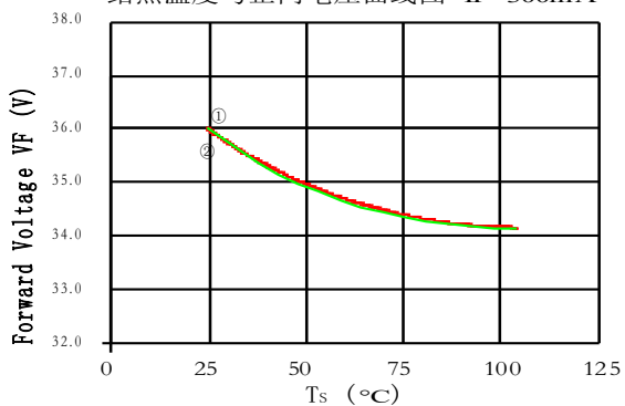
Case Temperature vs. Forward Voltage 结点温度与正向电压曲线图 IF=300mA
