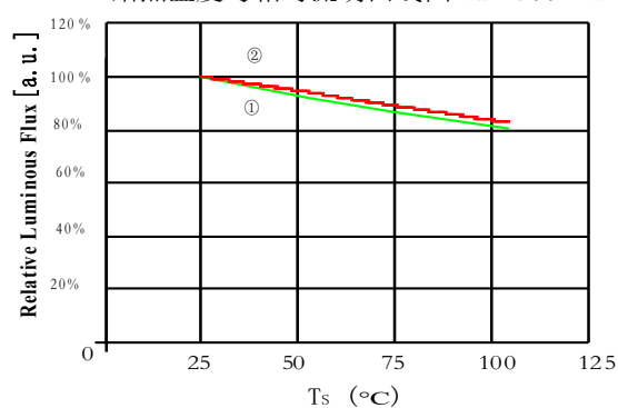
Case Temperature vs. Relative Luminous Flux 结点温度与相对流明曲线图 IF=300mA
