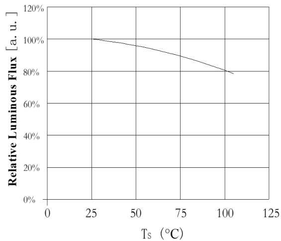
Case Temperature vs. Relative Luminous Flux 结点温度与相对流明曲线图 I_F = 960\text{mA}
