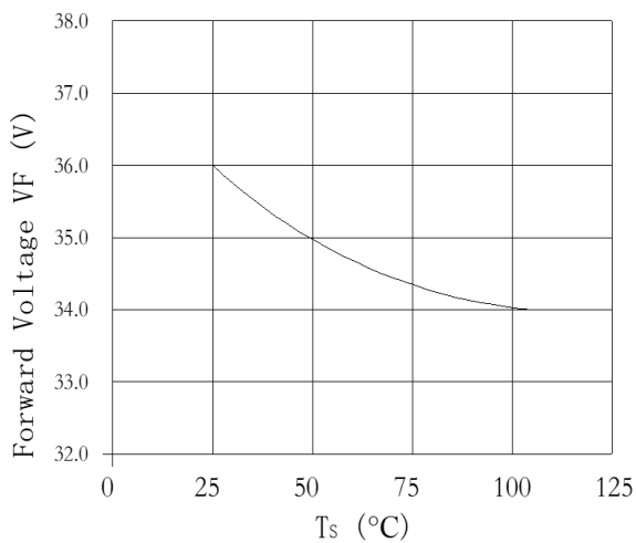
Case Temperature vs. Forward Voltage 结点温度与正向电压曲线图 I_F = 960\text{mA}
