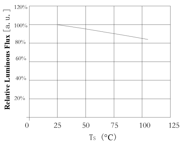
Case Temperature vs. Relative Luminous Flux 结点温度与相对流明曲线图 IF=750mA
