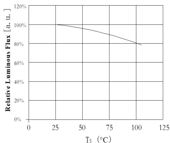
Case Temperature vs. Relative Luminous Flux 结点温度与相对流明曲线图 I_F = 280\text{mA}
