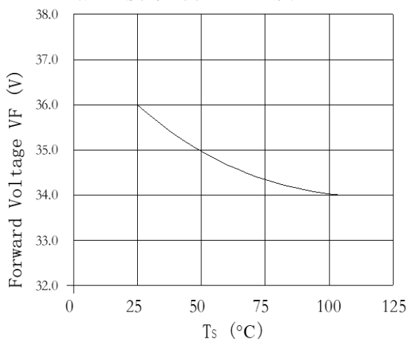
Case Temperature vs. Forward Voltage 结点温度与正向电压曲线图 I_F = 280\text{mA}
