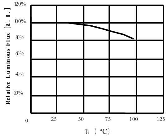
Case Temperature vs. Relative Luminous Flux 结点温度与相对流明曲线图 IF=200mA
