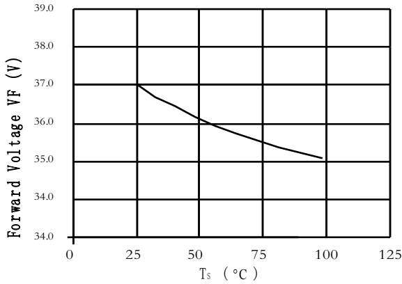
Case Temperature vs. Forward Voltage 结点温度与正向电压曲线图 I_F = 200\text{mA}
