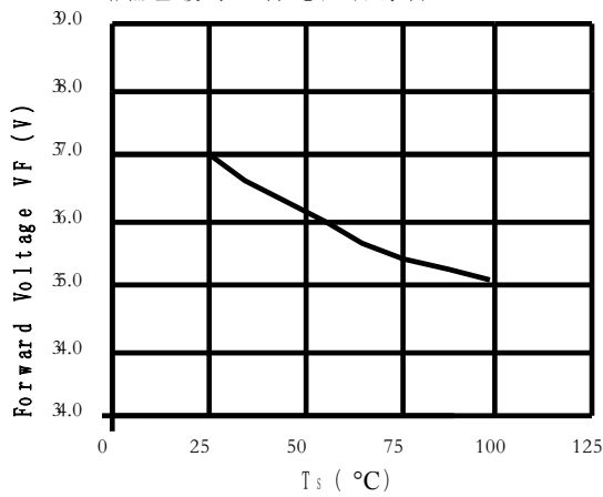
Case Temperature vs. Forward Voltage 结点温度与正向电压曲线图 IF=200mA
