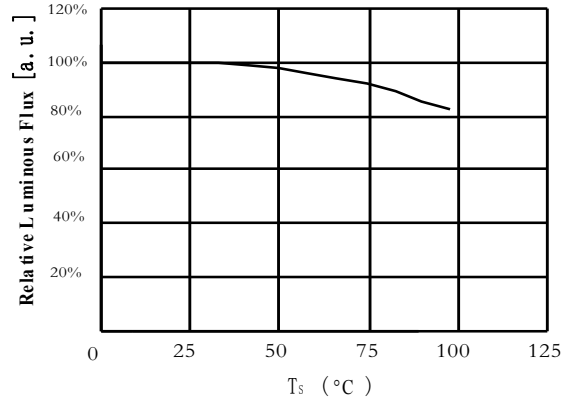
Case Temperature vs. Relative Luminous Flux 结点温度与相对流明曲线图 I_F = 200\text{mA}
