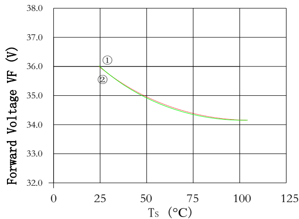
Case Temperature vs. Forward Voltage 结点温度与正向电压曲线图 I_F=300\text{mA}
