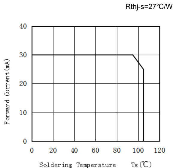
Soldering Temperature VS Allowable Forward Current 焊盘温度与允许温度电流特性
