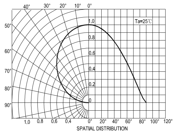
Radiation diagram
