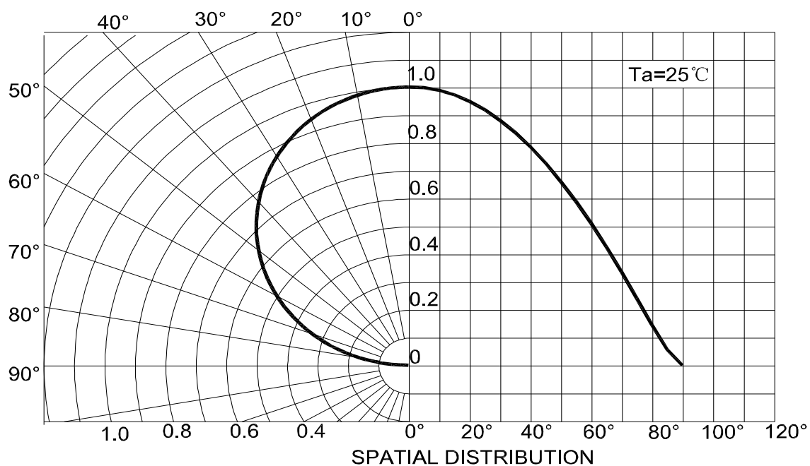
Radiation diagram
