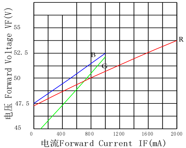
Forward Voltage vs. Forward Current 正向电压与正向电流曲线图 (R&G&B)
