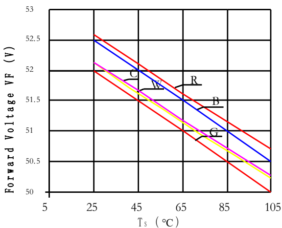
Case Temperature vs. Forward Voltage 结点温度与正向电压曲线图
