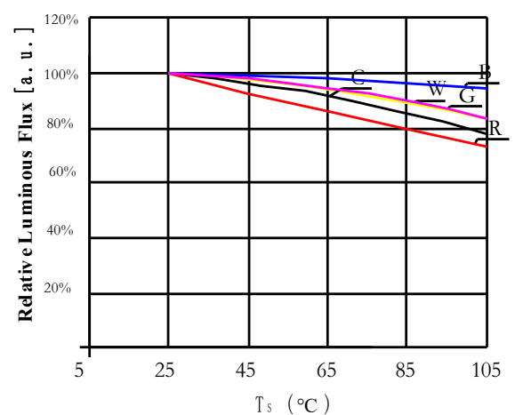
Case Temperature vs. Relative Luminous Flux 结点温度与相对流明曲线图
