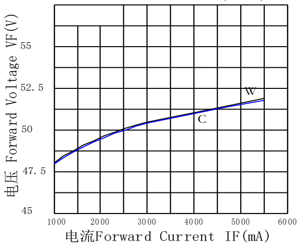
Forward Voltage vs. Forward Current 正向电压与正向电流曲线图(W&C)
