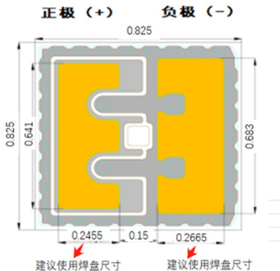
Chip Bottom View And Recommended Pad Size
