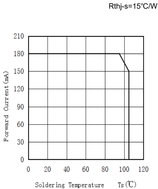
Soldering Temperature VS Allowable Forward Current 焊盘温度与允许温度电流特性曲线
