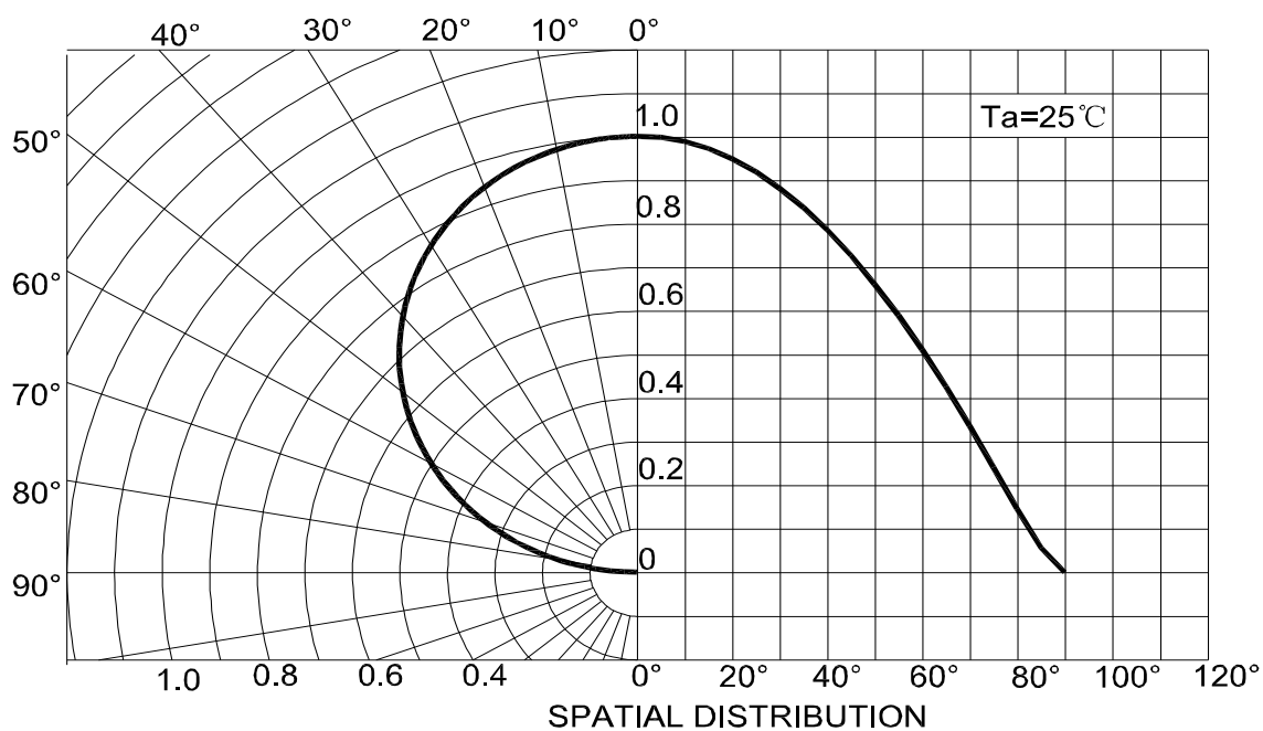
Radiation diagram
