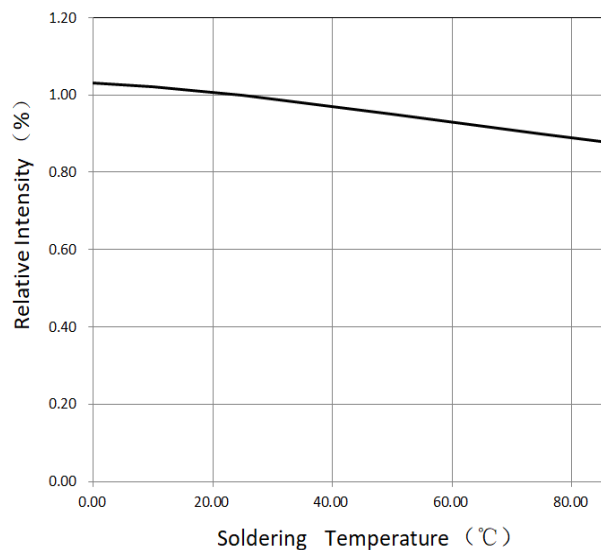
Soldering Temperature VS. Relative Intensity 焊盘温度与相对光强特性曲线
