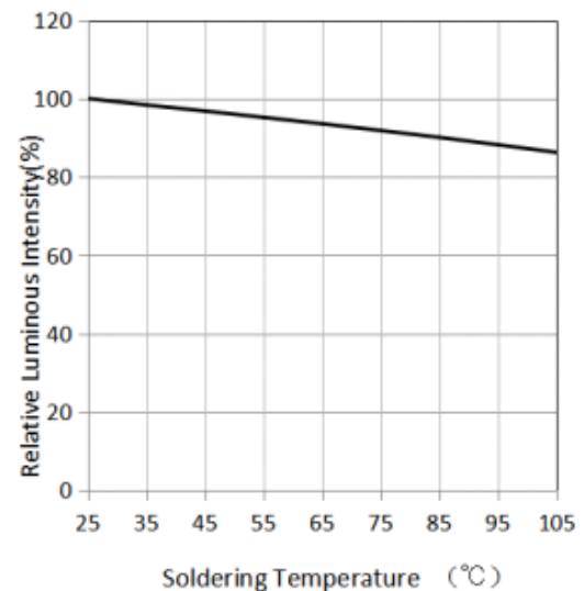
Soldering Temperature VS. Relative Intensity 焊盘温度相对光强特性曲线
