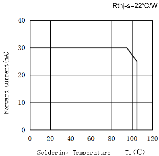
Soldering Temperature VS Allowable Forward Current 焊盘温度与允许温度电流特性
